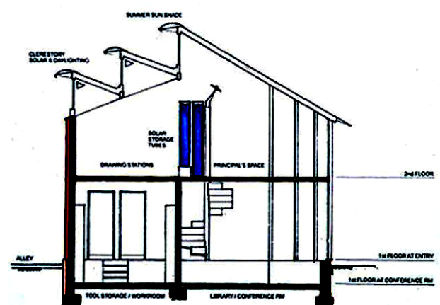
BUILDING SECTION
