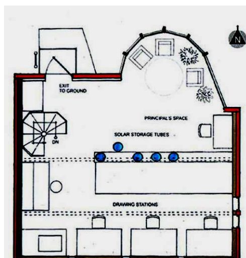
INTERIOR Energy Storing Materials: Water, Concrete, Masonry
